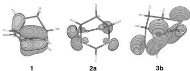
Figure 3. HOMOs of 1 , 2a , and 3b . The cyclopropane ring in 1 and 2a is on the left-hand side.
